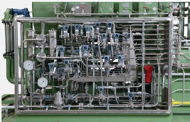
Gas seal transmitter rack with 2-of-3 voting, seal gas filtering and purge gas filtering
