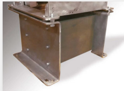
Pedestal Base Raises the MR150 off the rig floor. Includes pre-drilled bolt holes which match our legacy Man Rider and competitive products for securing to the rig floor.
