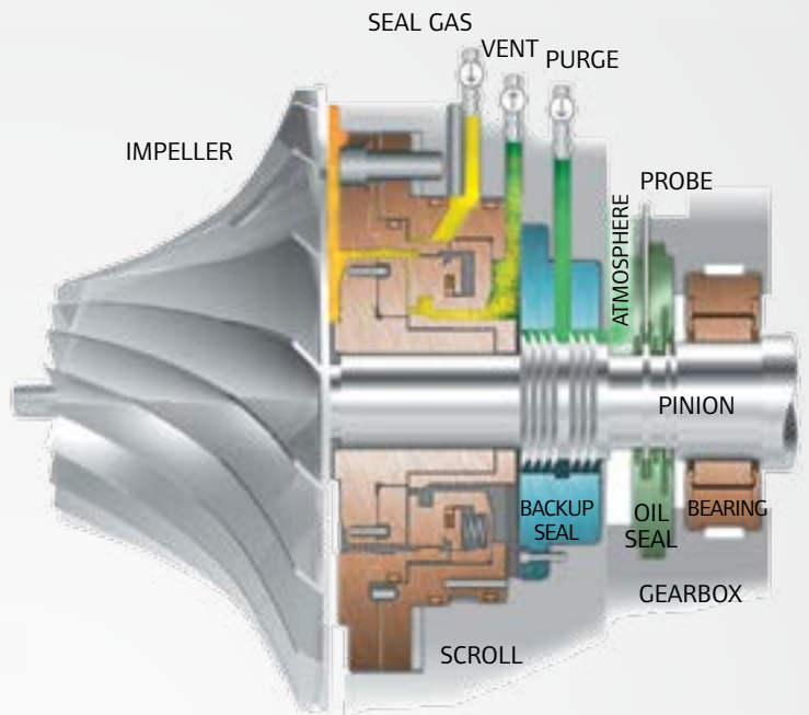
Single dry-face seal with a babbitted labyrinth backup
